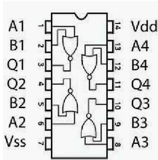
U2 CD4001 QUAD 2-INPUT NOR GATE
